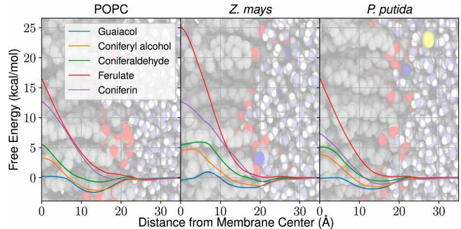
Free energy profiles of selected lignin-related compounds as a function of distance from the membrane center across a model membrane (left), a model plant membrane (middle), and a model P. putida membrane (right).
